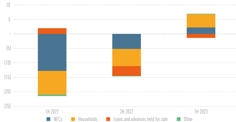
Figure 23: NPL cumulative net flows by segment for June 2022 to June 2023 (EUR bn) Source: EBA supervisory reporting data
