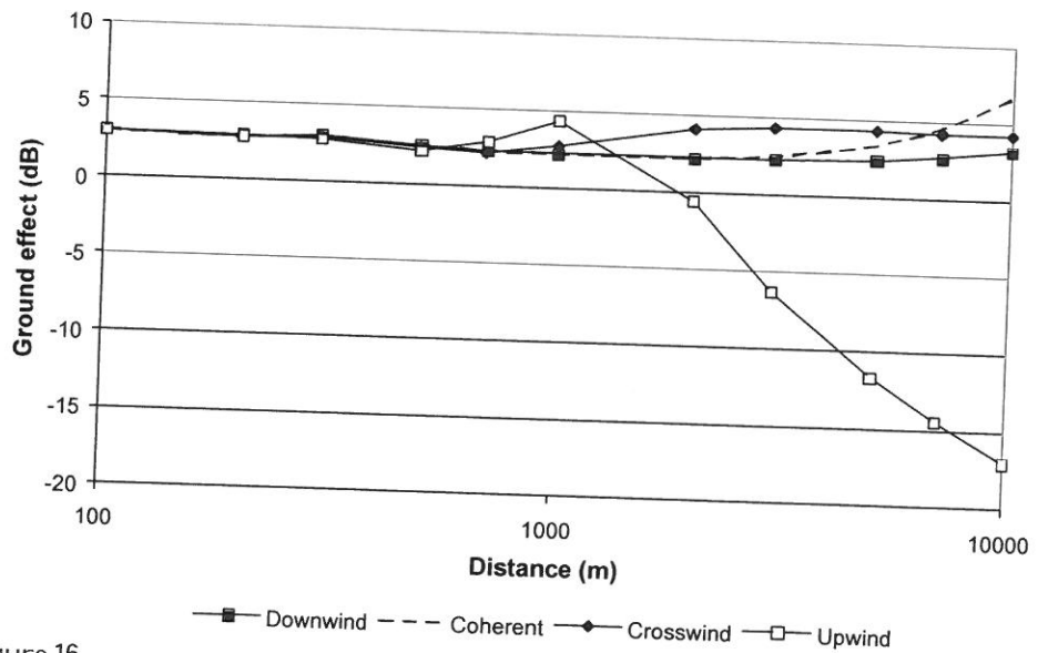
Figure 16 Ground effect for a wind turbine with a hub height of 100 m calculated with Nord2000 for different wind directions for propagation over water.
