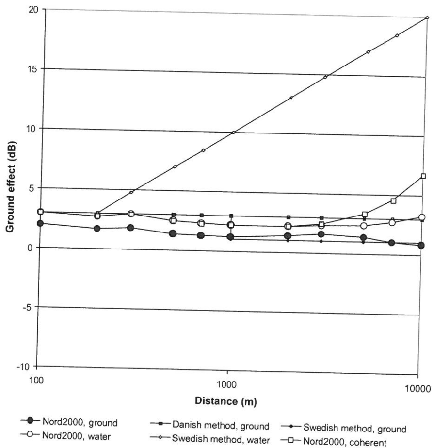
Figure 12 Ground effect for a wind turbine with a hub height of 100 m calculated according to different models at propagation both over ground and water.
