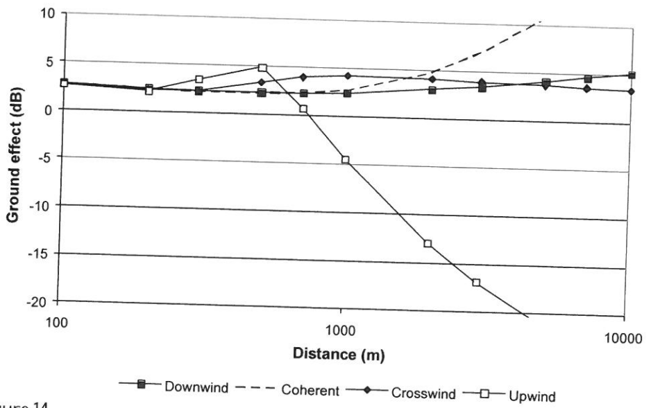
Figure 14 Ground effect for a wind turbine with a hub height of 30 m calculated with Nord2000 for different wind directions for propagation over water.
