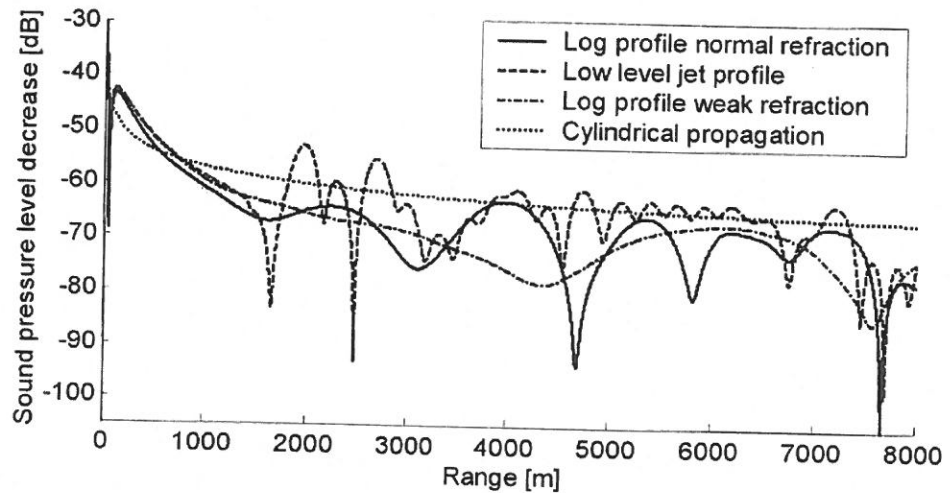
Figure 9 The decrease with distance of the sound pressure level from a 65 m high wind turbine at propagation over water under three different meteorological conditions and comparison with expected values assuming cylindrical propagation.
